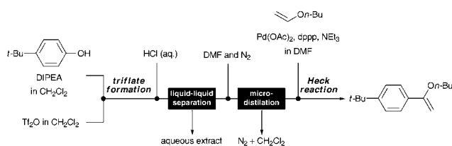
Scheme 7 Continuous synthesis of an enol-ether involving liquid-liquid separation and continuous solvent exchange (Jensen and Buchwald 20 ).
