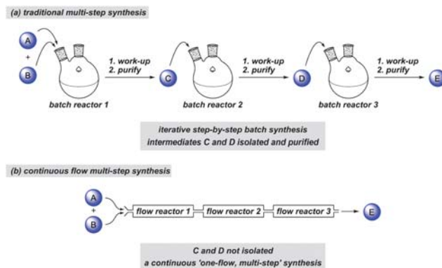
Fig. 1 Multi-step synthesis strategies.
