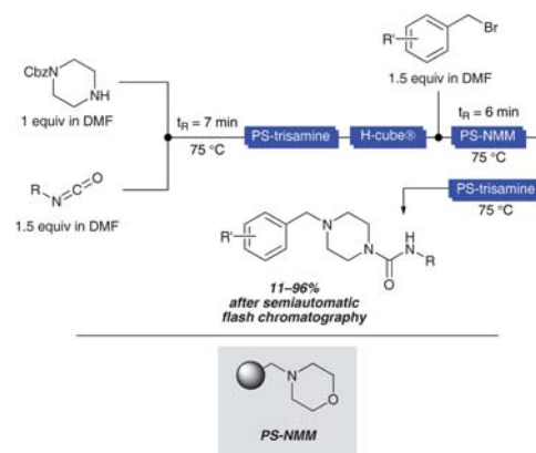
Scheme 12 Three-step continuous flow synthesis of receptor ligands (Ulven 34 ).
